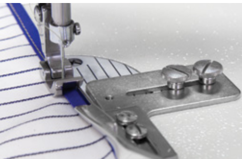
TEXI 4004 Universal screw for binders, hemmers and gauges (2 pcs)
