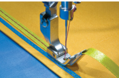
TEXI 5015 Foot with central tape guide 4.8 mm
